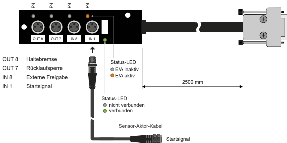
E/A-Expander 4/4 (4 Ports, Single) inkl. Kabel (MS-1002204)
