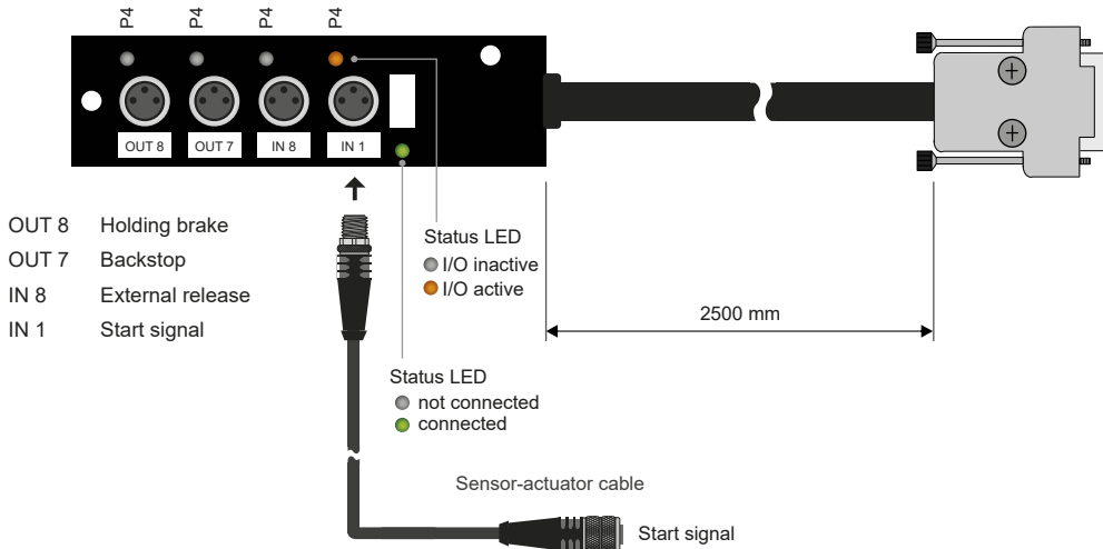
I/O Expander 4/4 (4 Ports, single) incl. cable (MS-1002204)
