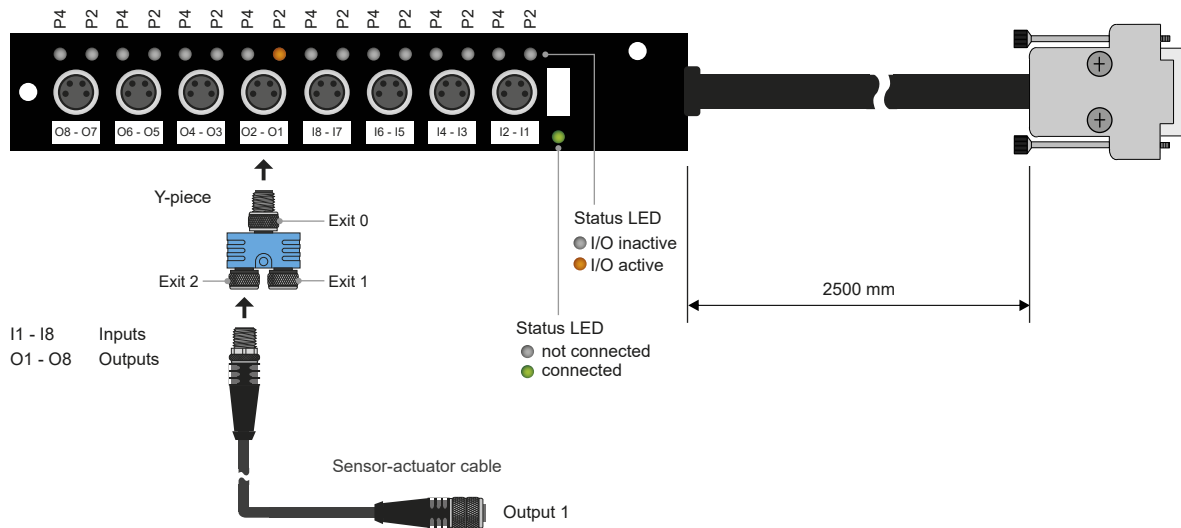
I/O Expander 8/8 (8 Ports, dual) incl. cable (MS-1002208)
